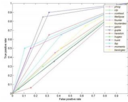
Figure 4. The ROC Curve: Crocodile VS Crocodile Head.
