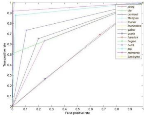
Figure 1. The ROC Curve: Airplanes VS Car Side.
