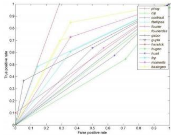
Figure 6. The ROC: Water Lilly VS Sunflower.
