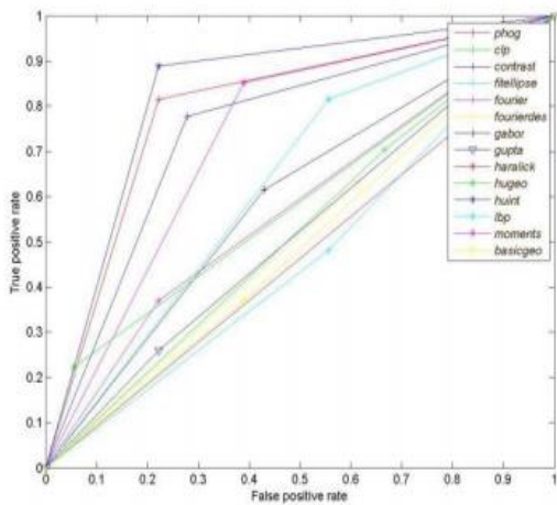
Figure 2. The ROC Curve: Cougar Face VS Cougar Body
