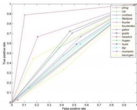
Figure 3. The ROC Curve: Crab VS Crayfish.
